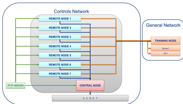
Figure 3: Block diagram of READS distributed network.
