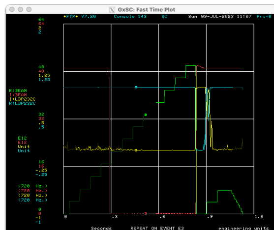
Figure 10: Real-time ML inferences on Fast Time Plot display - I:LDP232C and R:LDP232C are the loss percentage attribution for 232C BLM.
