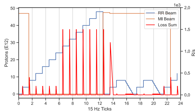
Figure 2: Example to overlay beam events and expected losses during a machine cycle.
