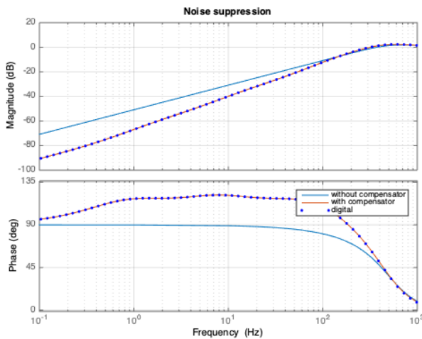
Figure 3: Noise suppression plot for closed loop.
