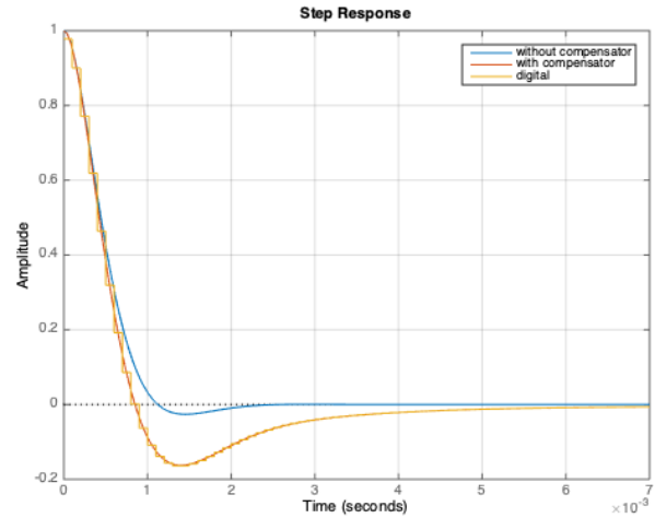
Figure 4: Transient response to the disturbance of the feedback system.
