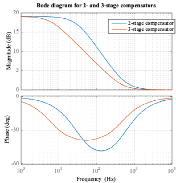
Figure 1: Bode plot of the open loop with two and three lag compensators. Total gain increase is the same but maximal phase shift different for three-stage it is 40° and for two-stage it is 50°.
