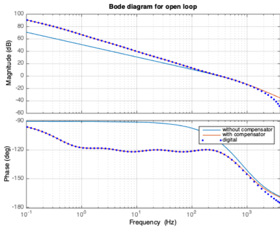
Figure 2: Example of the open loop gain with integrator and a pole at 800 Hz. Additional gain at low frequencies is about 20 dB, the phase margin is about 60° with and without compensator. Dots correspond to the digital system with 10 kHz sampling rate.
