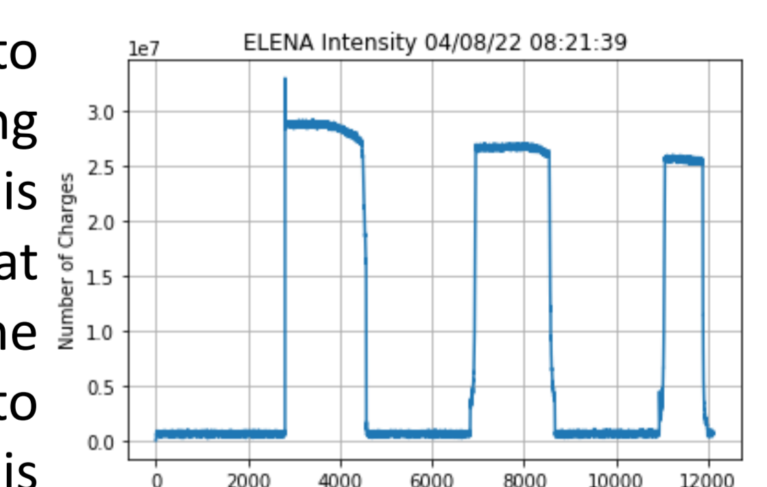
Figure 8: The Intensity IS measured in the bunched periods of the ELENA deceleration cycle
