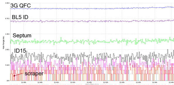
Figure 4: The loss rates in counts/second for different BLDs (in logarithmic scale) with the scrapers were parked.
