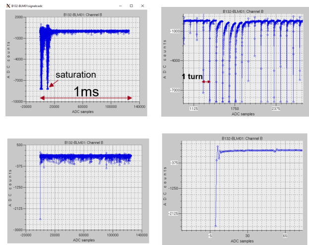
Figure 7: Raw ADC signals of the 3G-BLD for the injection beam loss (top left:the injection loss signal for 1 ms; top right: zoomed in) and the life time beam loss (bottom left: lifetime loss signal for 1 ms; bottom right: zoomed in).
