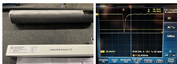
Figure 1: Libera BLD with the lead sleeve (left) and the analog signal for background cosmic ray detection (right).
