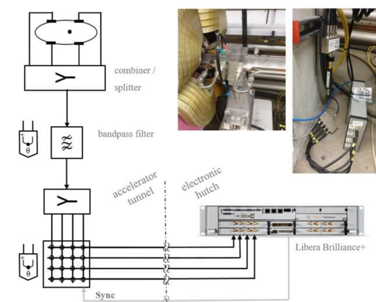
Button BPM test setup with external crossbar-switching (ECS) frontend and adapted Libera Brilliance+ (**) readout electronics.
