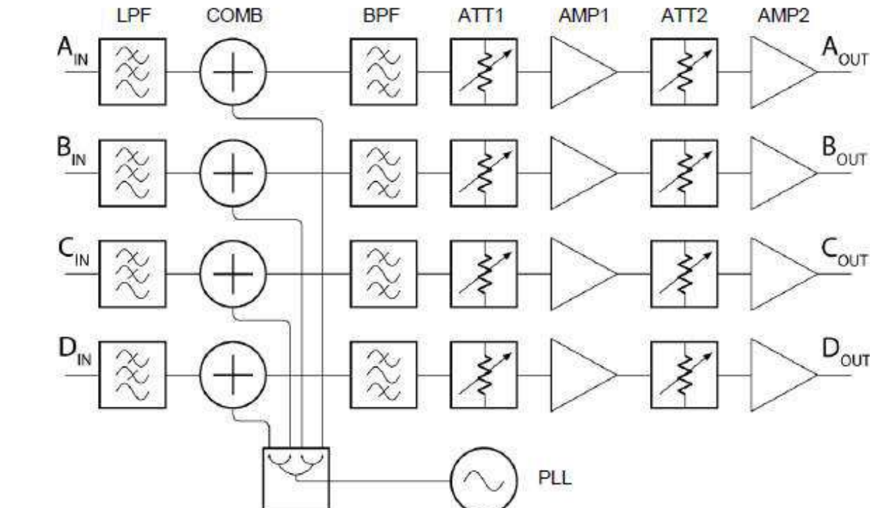
ELETTRA BPM Pilot-Tone (PT) frontend (*)
