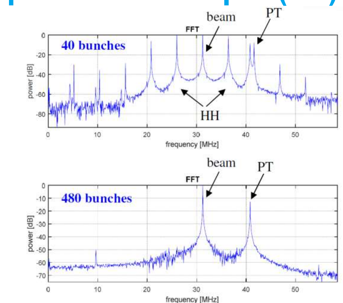
Typical amplitude spectra of a PT system used for PETRA III test measurements at 40 bunch/100mA and 480 bunches/120mA beam modes (HH: higher harmonics).
