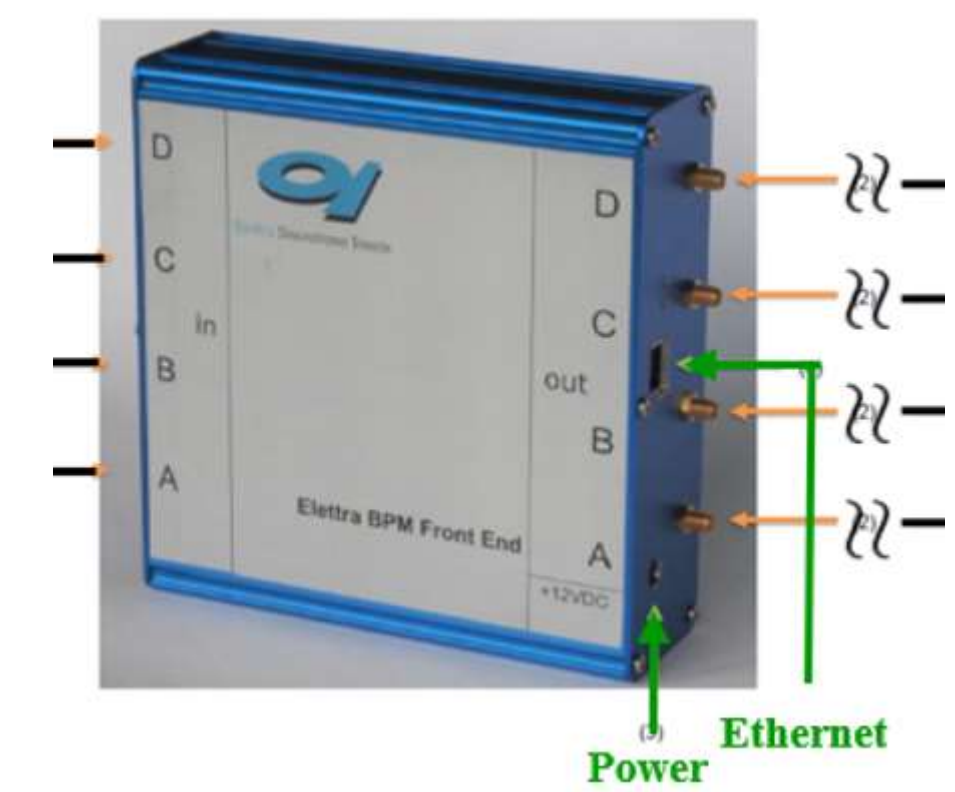
The ELETTRA BPM Pilot-Tone frontend box (*)
