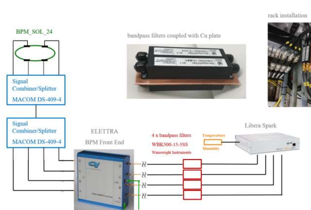
Button BPM setup with PT frontend and adapted Libera Spark (**) readout electronics
