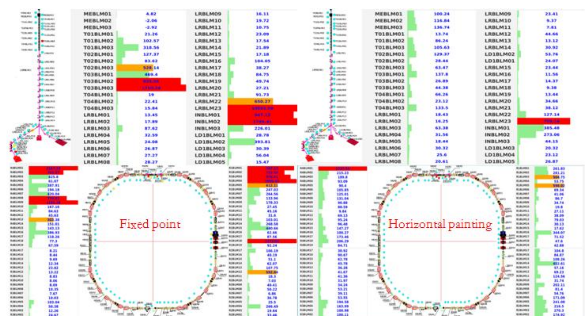
Fig. 4: Beam loss of the Linac and RCS while the fixed point injection (left) and horizontal painting injection (right) were used.
