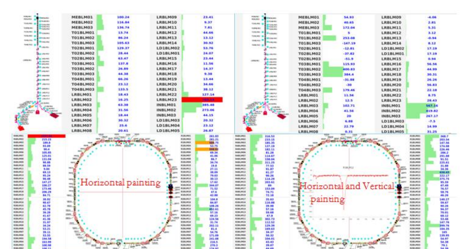
Fig. 7: Beam loss of the Linac and RCS while the horizontal painting injection (left) and horizontal & vertical painting injection (right) were used.
