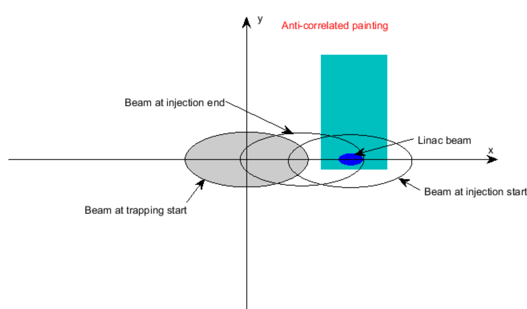
Fig. 3 Positions of the ring acceptance ellipse during the horizontal painting injection.
