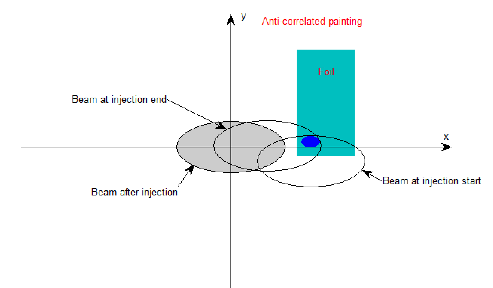
Fig. 6: Positions of the ring acceptance ellipse during the horizontal and vertical painting injection.
