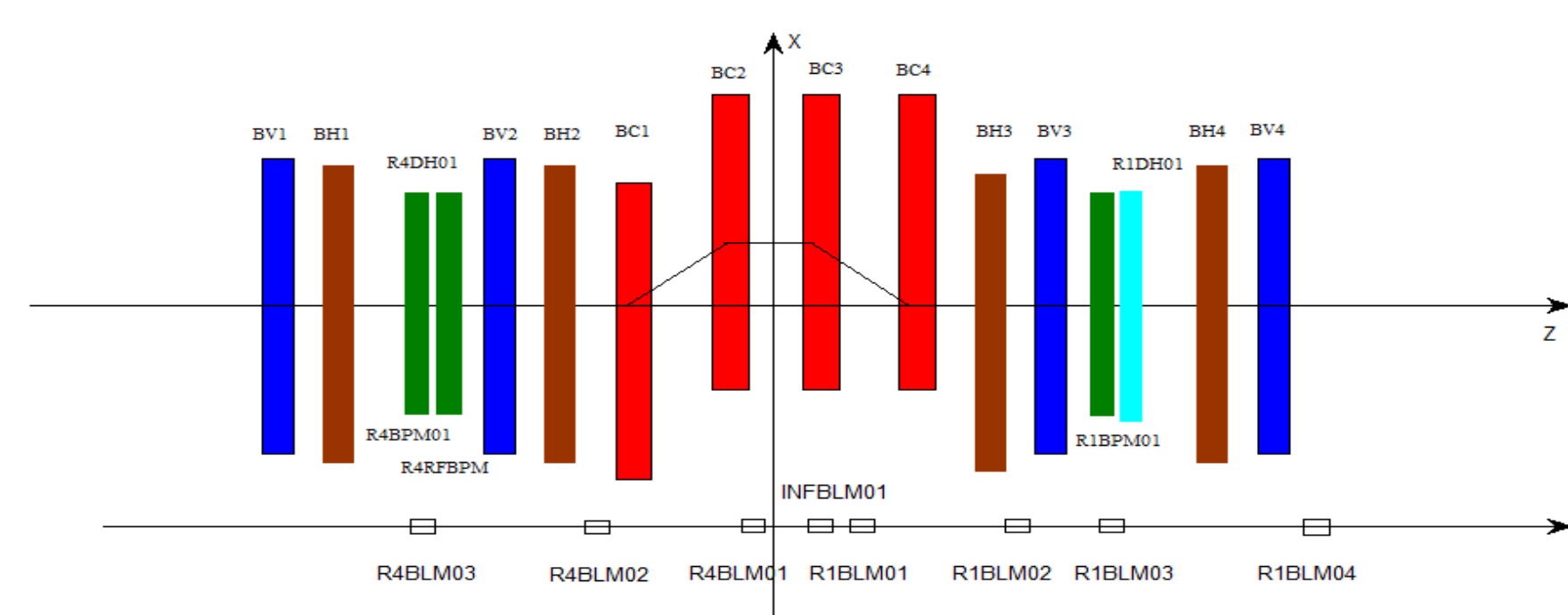
Fig 2: Layout of CSNS injection system.
