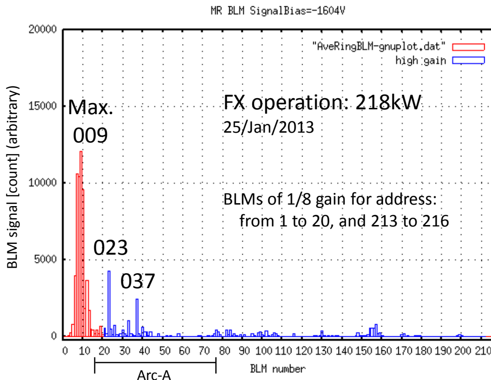
Typical beam loss distribution
