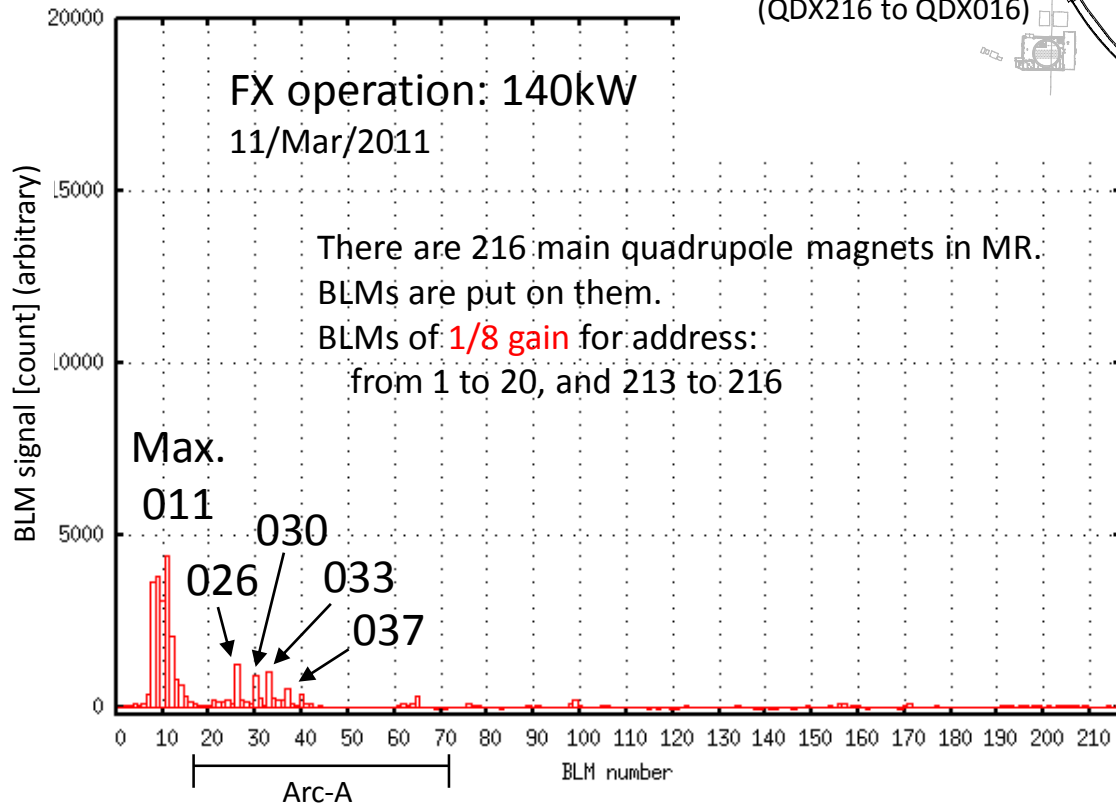
Typical beam loss distribution
