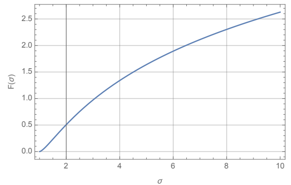
Figure 1: The function F(\sigma) .
