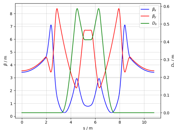
Figure 3: Lattice functions in one cell for an operation mode with nominal momentum compaction of 14.8 \times 10^{-3} . The dispersion is located between the dipoles and does not exceed 0.6 m, while the momentum acceptance is about \pm 4\% .
