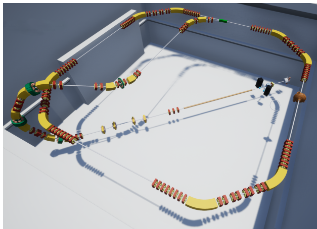
Figure 1: Artistic view of the cSTART project. The cSTART storage ring at a height of about 3.5 m is connected to the FLUTE injector by a complex 3D transfer line. The LPA (not shown) will be at the same height as the storage ring and uses the last part of the transfer line of FLUTE for injection.
