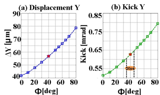
Figure 5: Vertical displacement at z = 0.3 m and kick strength as a function of the gun phase.
