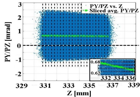
Figure 8: Bunch distribution at z \approx 0.33 m in terms of the vertical kick strength versus z -positions.
