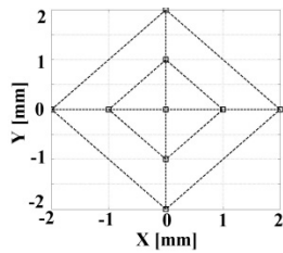
Figure 6: Beam centroid positions on the cathode plane used in the simulations for kick quantification.
