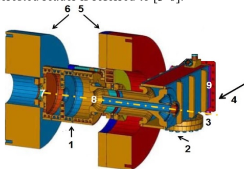
Figure 1: Sketch of the PITZ gun with coaxial RF coupler: 1-gun cavity, 2-door-knob transition, 3-cavity axis, 4-RF feeding direction, 5-main solenoid, 6-bucking solenoid, 7-cathode, 8-end of coaxial line and 9-reference position of WG port for simulations. Note that this sketch is rotated by 90 degrees compared to the computational model used in the follow-up simulations.
