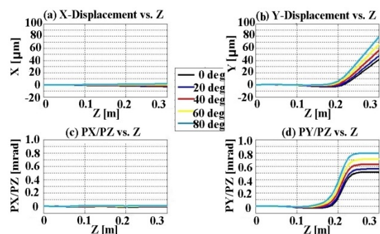
Figure 4: Off-center distance on the transverse plane and corresponding transverse momentum of the beam centroid for the RF start-phases.
