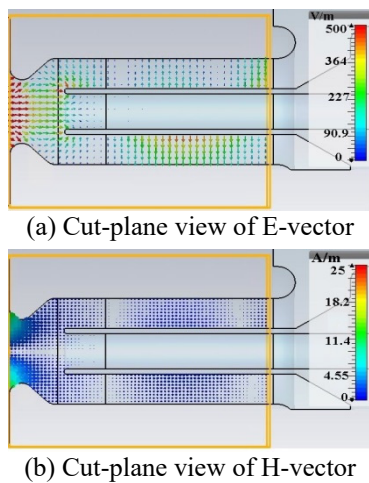
Figure 2: Illustration of the local RF field asymmetries. The colour maps are adjusted for a better visualization.
