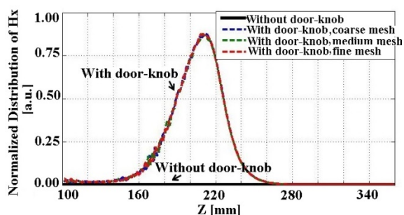
Figure 3: Distribution of the magnetic field component along the cavity axis and the comparison with the same field calculated by a simulation without the door-knob transition and the rectangular waveguide in the computational model. Different curves in colours represent gradual steps for mesh refinements in the simulations.
