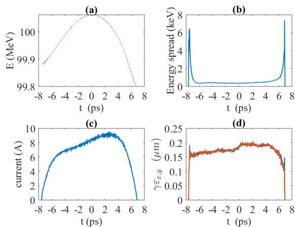
Figure 3: Electron longitudinal phase space, beam current, slice energy spread and slice emittance at injector exit for SCRF gun setup.
