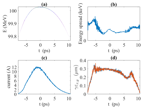
Figure 2: Electron longitudinal phase space, beam current, slice energy spread and slice emittance at injector exit for NCRF gun setup.
