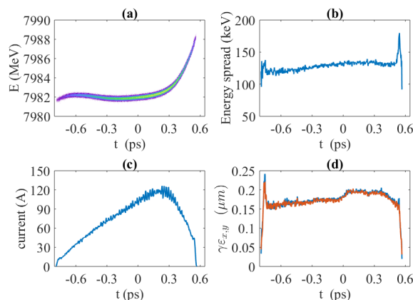
Figure 5: Electron longitudinal phase space, beam current, slice energy spread, and slice emittance after linac optimization, using SCRF injector beam.
