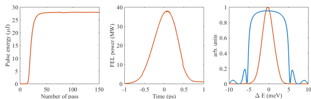
Figure 6: XFELO performance for 14.4 keV using 0.25 \mu\text{m} emittance, 130 keV slice energy spread and over 500 fs flat part beam with the SCRF gun setup.
