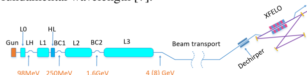
Figure 1: Layout of the proposed XFEL at the LCLS-II.
