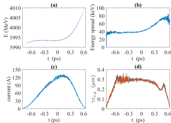
Figure 4: Electron longitudinal phase space, beam current, slice energy spread, and slice emittance after linac optimization, using NCRF injector beam.
