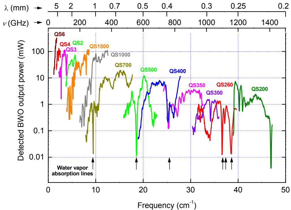
Fig. 2: Output power and spectral distribution of BWO devices employed in a CW spectroscopic system at the 1st Physics Institute of the University of Stuttgart. (Courtesy of M. Dressel, University of Stuttgart)
