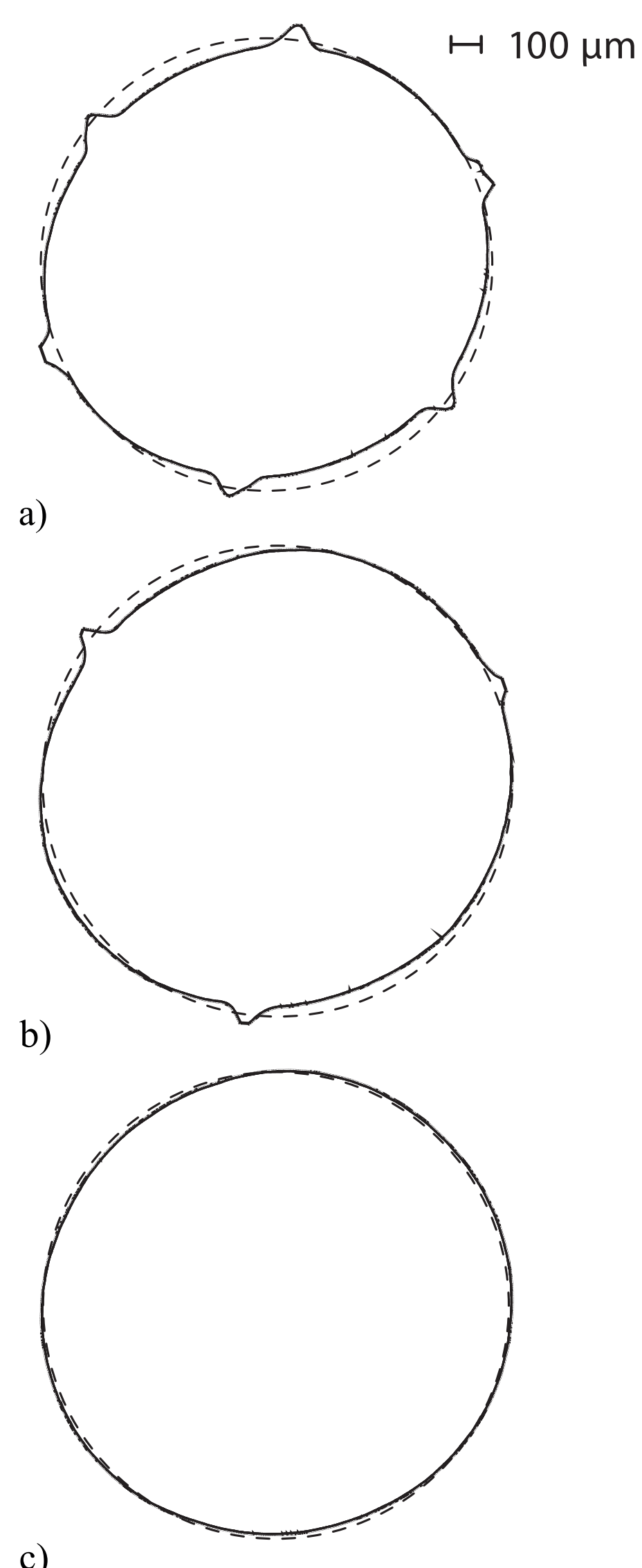
The measured deviation of the plasma chamber surface from the ideal circle (dashed). The values are amplified by a factor 100. The inner diameter of the chamber is 78 mm. The measurement was taken a) roughly in the middle of the chamber, b) at around a quarter of the chamber length and c) at the extraction end of the chamber.
