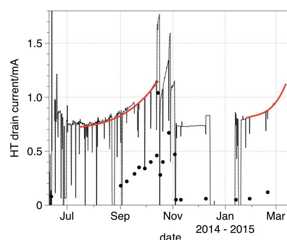
The current of the extraction power supply. The dotted line is the total current when the plasma is on, the dots show some selected values of the drain current when the plasma is off. The red curve represents a cubic fit of the current. In November there was the source maintenance. Due to the clean insulators the drain current dropped down, but over time started to rise again.
