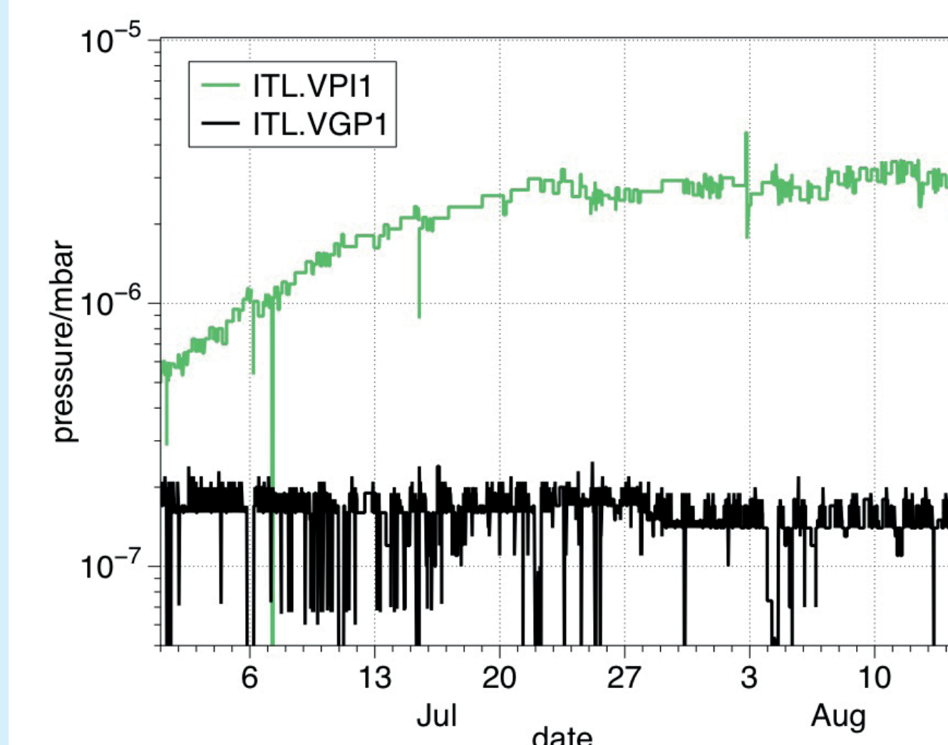
Vacuum measured in the LEBT with a Penning gauge (ITL.VGP) and in one of the ion getter pumps in the LEBT (ITL.VPI). The current measured in the ion getter pump is taken as measure for vacuum pressure.
