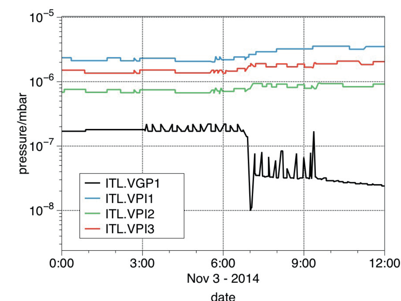
Vacuum measured in the LEBT with a Penning gauge (ITL.VGP) and in the ion getter pumps (ITL.VPI). At 7:00 the LEBT was separated from the source with a valve.
