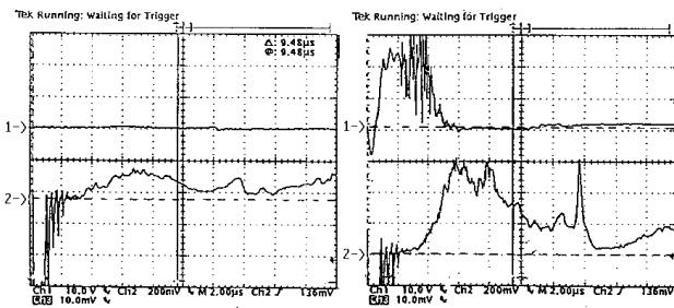
Figure 2a (left) and b (right): Trace 1 - Thermoelectron current. Trace 2 - Faraday cup signals, without (left) and with (right) thermionic cathode heating. Target and expansion area: 60 kV; acceleration electrode: -20 kV; deceleration electrode: 0 kV; Faraday cup electron suppression grid: -1 kV; thermionic cathode grid potential: -1.5 kV.
