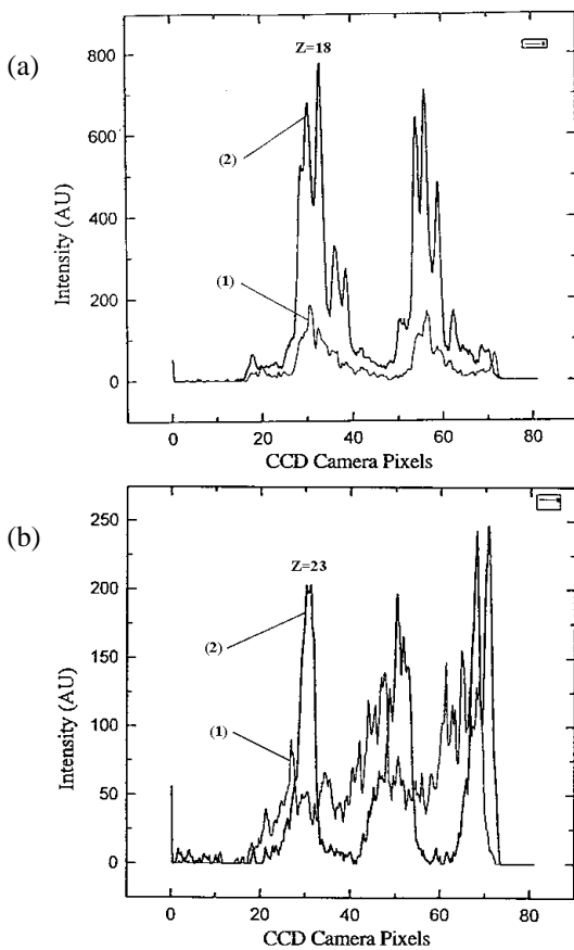
Figure 4: Integrated plots of CCD images around a) z = 18 and b) z = 23 . Trace 1 without thermoelectrons, Trace 2 with thermoelectrons.
