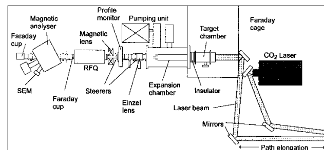
Figure 1: Schematic diagram of the CERN Laser Ion Source experimental apparatus.
