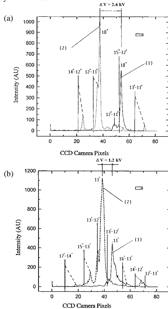
Figure 3: Integrated plots of CCD Image around a) z = 10 and b) z = 11 . Trace 1 without thermoelectrons, Trace 2 with thermoelectrons.
