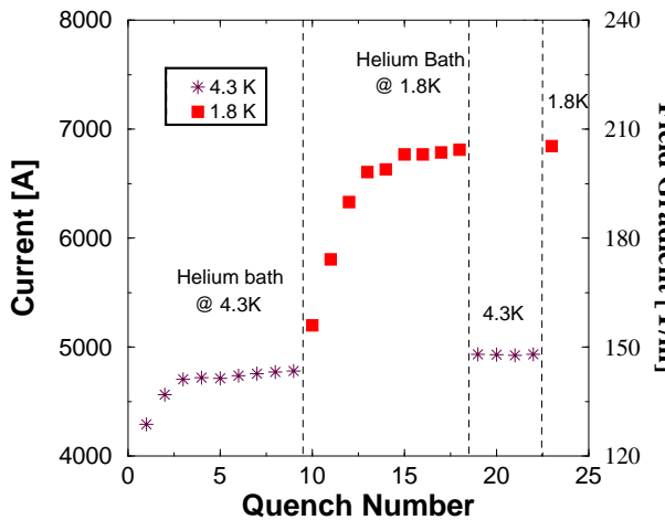
Figure 2: Quench training history for R54001.
