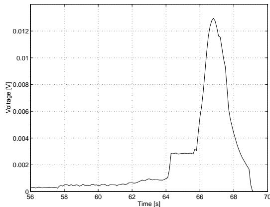
Figure 5: Voltage V_MBB(SSS) (see Figure 3) versus time for a quench at 7 kA
