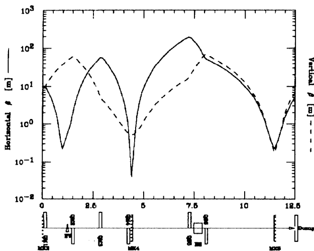
Figure 2: \beta -Functions for High- \epsilon in Figure 1 and Table 1.
