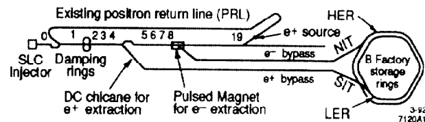
Fig. 1. Schematic of the B Factory e ± injection system, using the SLC linac and added bypass lines.
