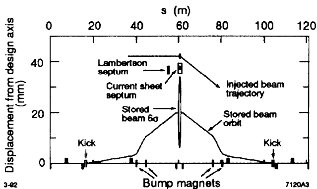
Fig. 3. Stored beam orbit during injection into HER. Applies also to LER with a change of scale.
