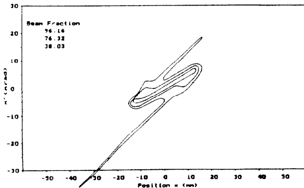
Figure 9. The emittance of a 30mA H - beam
