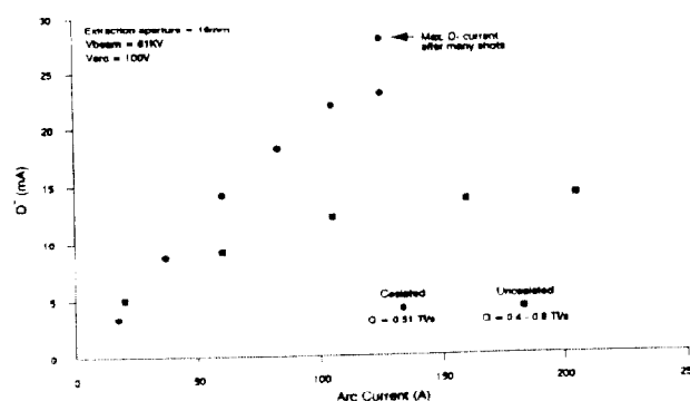
Figure 8. D + current with the addition of cesium
