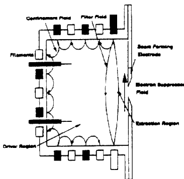
Figure 1. Schematic volume ion source
