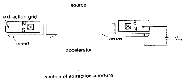
Figure 3. The electron suppressor
