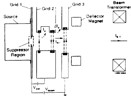
Figure 2. The triode accelerator
