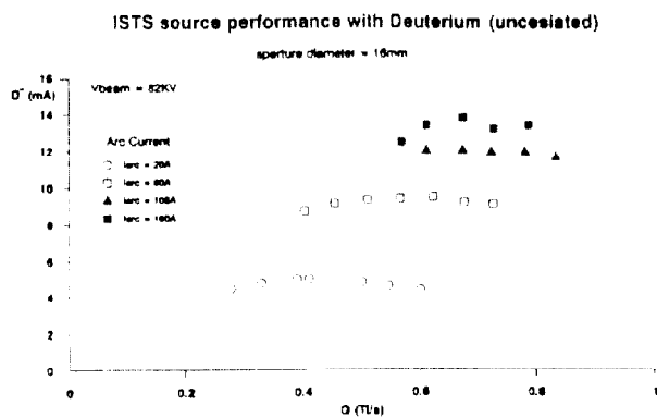
Figure 6. D + current as a function of gas flow
