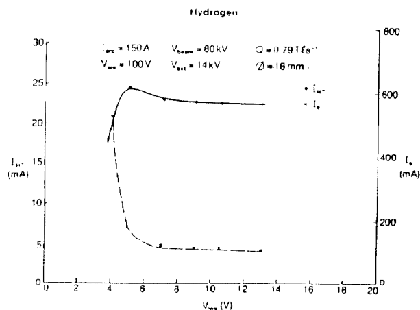
Figure 4. The action of the electron suppressor
