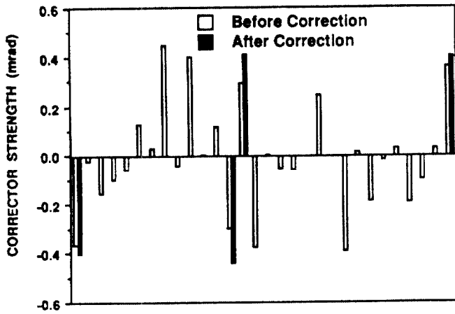
Figure 3. Vertical corrector pattern in SPEAR before and after correcting for misalignment errors at the Interaction Regions.
