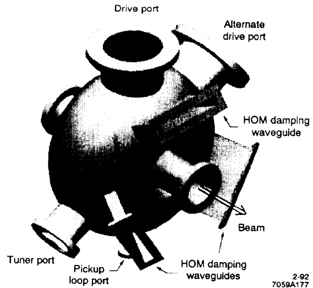
Fig. 2. Low-power PEP-II RF cavity prototype.
