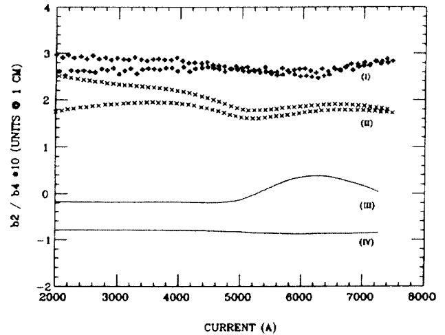
Fig.2 Excitation Behavior of b_2 and b_4 (I): measured b_2 , (II): measured b_4 , (III): calculated b_2 , (IV): calculated b_4 in DSA326
