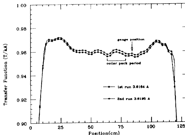
Fig.1 Transfer Function Distribution. ESR measurement results from magnet DSA324. The iron yoke was previously magnetised in opposite direction.
