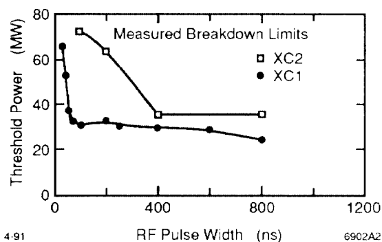
Figure 2. Performance of the first SLAC X-Band klystrons.
