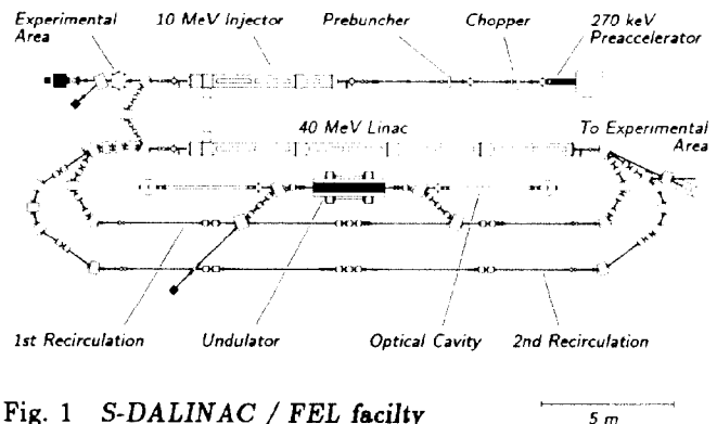
Fig. 1 S-DALINAC / FEL facility
