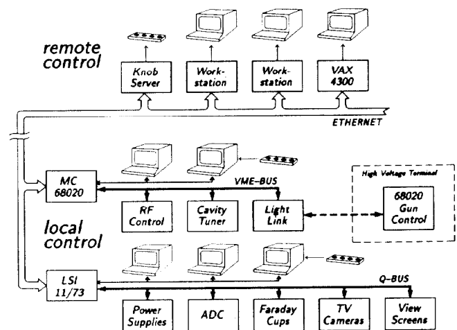
Fig. 2 S-DALINAC control system
