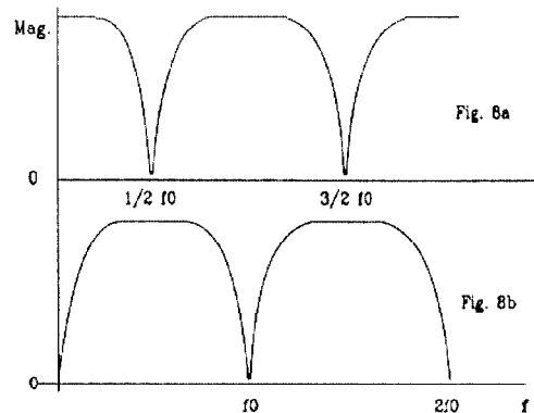
Amplitude versus frequency notch filter response. The f0 period is defined by the length of the delay line ( fig. 7b ) or by 2 times the length of the cable ( fig. 7a).
