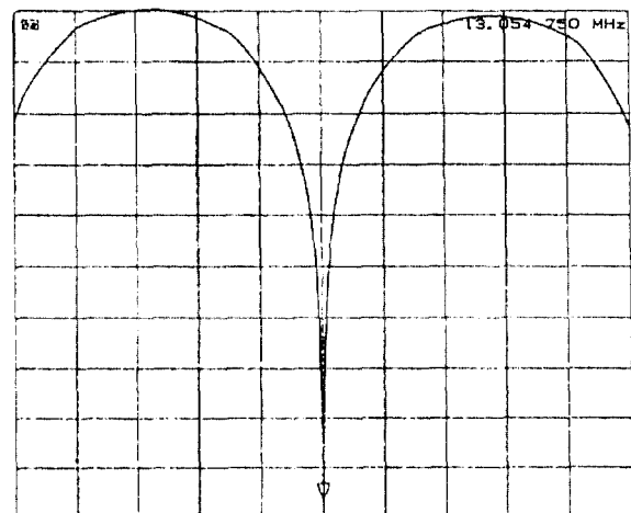
Fig. 12 Digital notch behavior. 5dB/div, frequency span 400 KHz Centre frequency 13.054 MHz.
