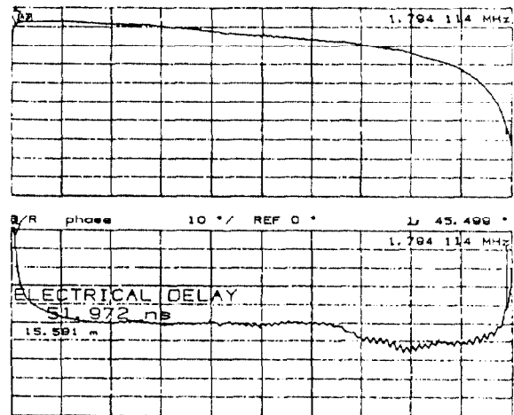
Fig. 10 Amplitude and phase versus frequency digital delay line response 5 dB/div, 10°/div, sweep 0.3-200 MHz.
