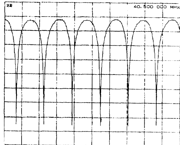
Fig. 11 Periodic digital notch effect . 5dB/div, frequency span 1 MHz. Centre frequency 40 MHz.
