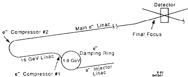
Fig. 1. Schematic of a Next Linear Collider.
