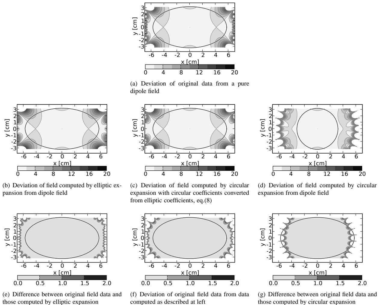
Figure 1: Test of the interpolation for the CSLD8b at a current of 873 \text{ kA} and a field of \approx 0.13 \text{ T} . The field B_y in the aperture is plotted. The gray indicates the absolute value of the deviation (in units). The original data are given on top. The upper row shows the data as reconstructed using the interpolation and the lower columns shows the absolute value of the difference between the reconstructed and the original data.
