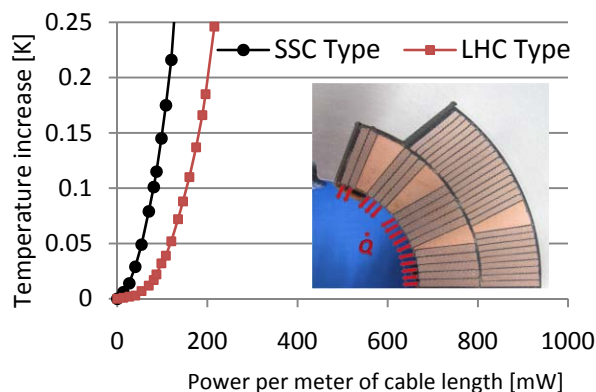
Figure 2: Temperature increase of an insulated cable transferring heat into a superfluid helium bath at 1.9 K through its inner edge. Data scaled from [2].
