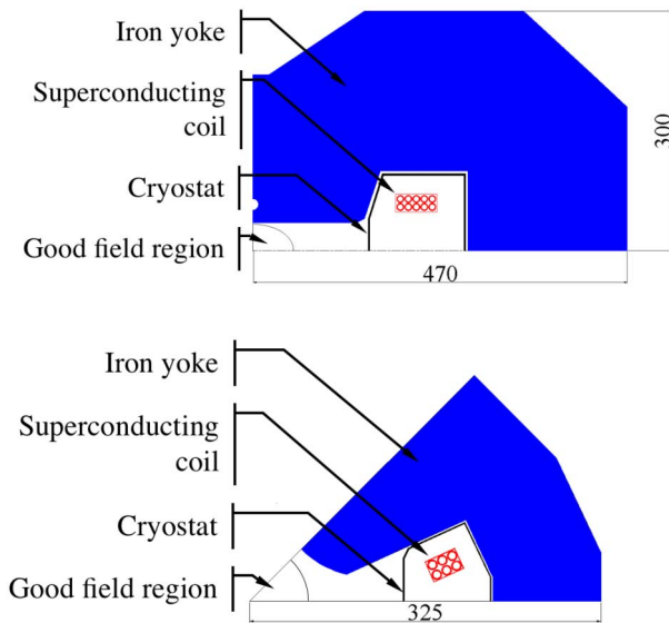
Figure 1. Schematic 1/4 cross section of the superferric dipole and 1/8 of the quadrupole designed for PS2.
