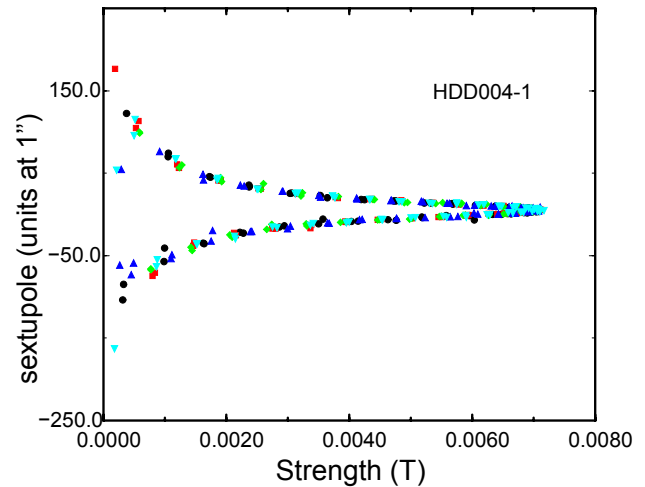
Figure 4: The measured sextupole vs the dipole strength, in case of 16 Hz AC, for different probe rotations, represented with the different color points. Every probe rotation produces 64 independent measurements for different magnet strength.
