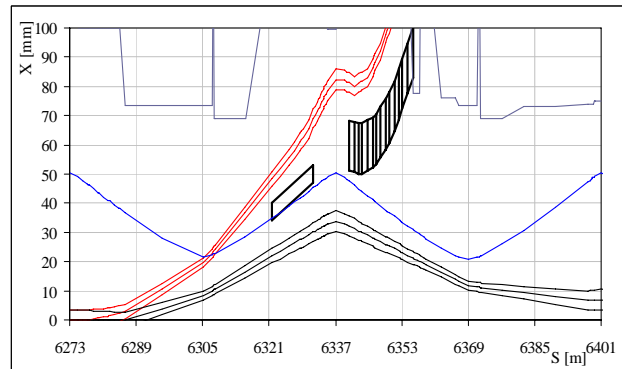
Figure 1: Extraction region in LSS6, showing the injected 5σ CNGS beam envelope (blue), the bumped 4σ LHC beam (black) and the extracted 4σ LHC beam (red).
