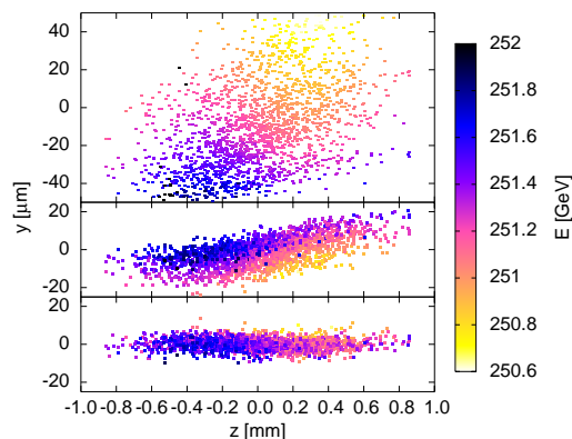
Figure 1: Example of tuning bumps in the ILC linac. The beam is plotted in the z - y plane, with color corresponding to energy, for different correction methods. Top plot shows beam after one-to-one correction. Middle plot shows the beam after Dispersion Free Steering (DFS), while the bottom plot shows the beam after DFS and optimization of emittance tuning bumps.
