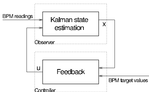
Figure 2: Block diagram of the Kalman Filter orbit correction feedback loop.
