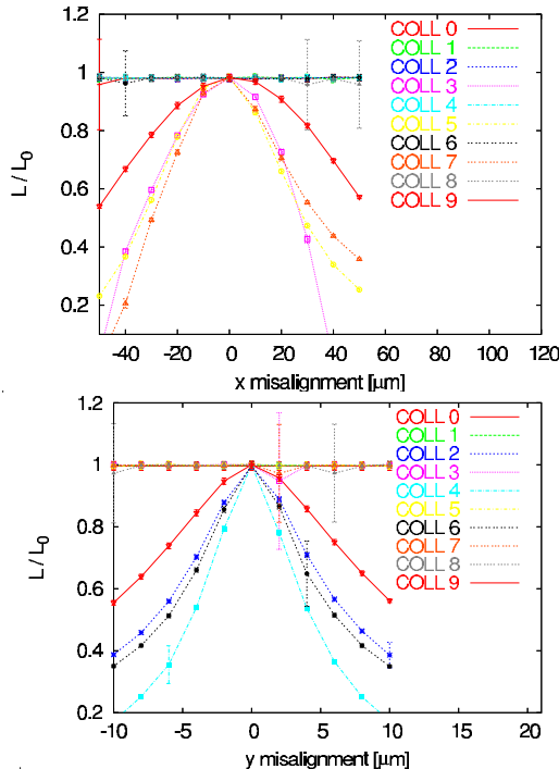
Figure 4: Luminosity reduction curves due to horizontal and vertical misalignment of collimators in the CLIC BDS.
