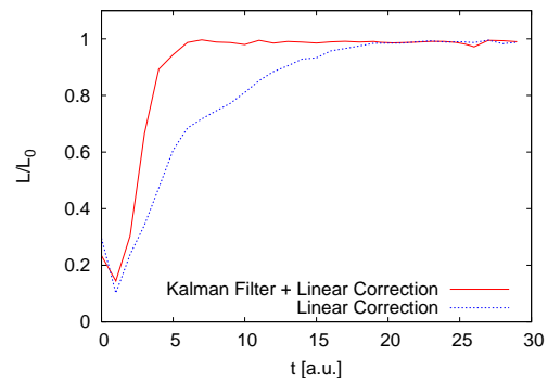
Figure 3: Kalman Filter+Linear Solver vs standard Linear algorithm, recovering the luminosity of a CLIC BDS subject to ground motion. Notice that KF+LS convergence is faster than plain LS.
