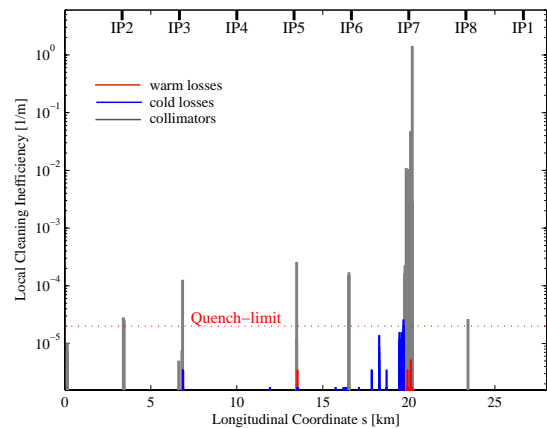
Figure 1: Proton loss map for Beam 2 betatron cleaning at 7 TeV (horizontal halo). The full phase 1 collimation system is simulated with collision optics. Blue bars correspond to losses on SC elements, red bars to losses in warm elements and grey bars to inelastic interactions in collimators. The beam moves from the right to the left. The estimated quench limit refers to nominal intensity ( 3.2 \times 10^{14} protons) and 0.2 hours beam lifetime.
