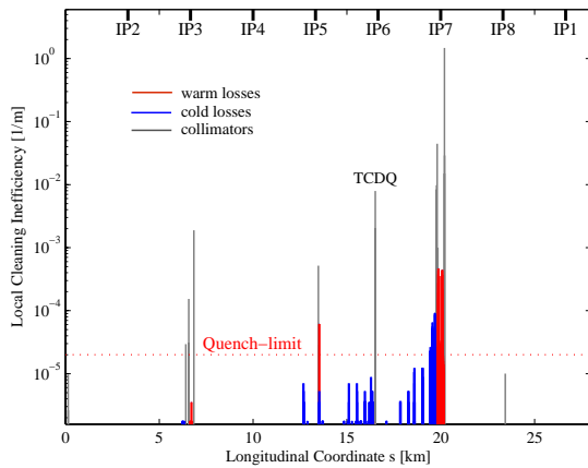
Figure 4: Loss map for scenario 2b and for Beam 2.
