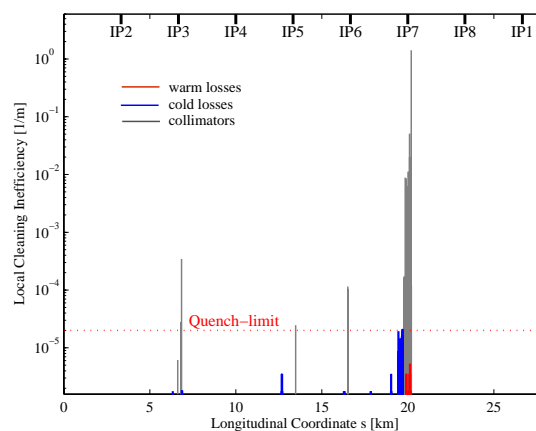
Figure 2: Loss map for scenario 0 and Beam 2.
