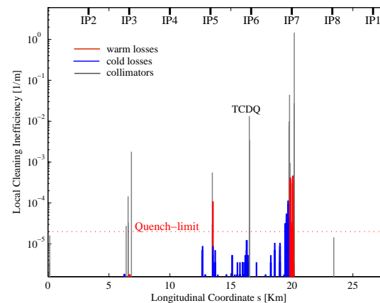
Figure 3: Loss map for scenario 2a and for Beam 2. The bar corresponding to particles absorbed on TCS@TCDQ is a factor 100 higher than for the nominal case (see Fig. 1). Losses in SC magnets (cold) appear immediately after the TCDQ but are below the quench limit.
