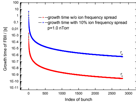
Figure 1: The growth time of FBII at OCS damping ring, 10% of ion angular frequency spread is considered.
