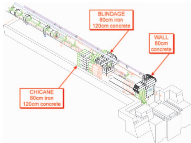
Figure 3: Layout of the shielding at the IR7 side of IR8.
