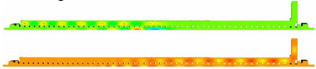
Figure 6: (Top) Eigenmode with low kick factor/high Q from Omega3P in 1 st band of the H60VG4, and (bottom) eigenmode with high kick factor/low Q in same structure.
