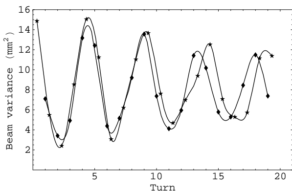
Figure 1: Horizontal beam width oscillations measured with the quadrupole pick-up (stars) and a SEM-grid (diamonds). The lines are spline interpolations.
