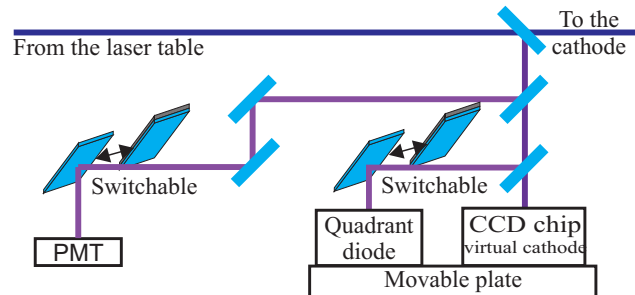
Figure 1: Optical scheme of the laser beam stability diagnostics
