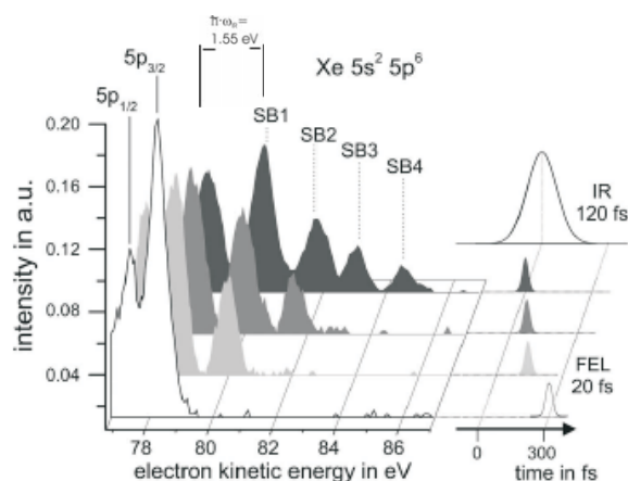
Figure 3: (Figure adapted from [6]) Time of flight spectra of Xe photo electrons with varying temporal overlap between the optical and XUV laser pulse.
