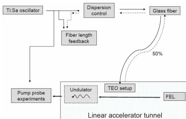
Figure 1: Overview of the principle setup of the TEO experiment. The relative arrival time between FEL pulse and IR pulse is measured inside the accelerator tunnel using the electron bunches instead of the XUV pulses.
