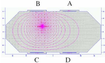
Figure 3: Cross section of the SESAME vacuum chamber, pick up buttons with a non-centered beam. Figure 3 shows the vacuum chamber cross section and the BPM Pick up's. The electrical beam position in the horizontal/ vertical plane is given by:
