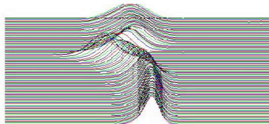
Figure 1: 108 consecutive horizontal profiles of a bunch of 6 \times 10^{10} protons accelerated in the SPS.
