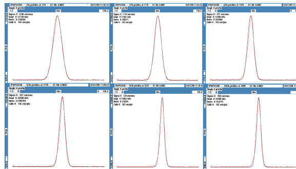
Figure 2: Six horizontal individual bunch profiles of a bunch of 6 \times 10^{10} protons accelerated in the SPS.
