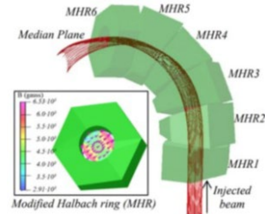
Magnetic inflectors
