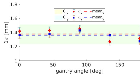
Figure 4: Measured beam size ( 1\sigma ) as a function of the gantry angle. The dashed line is the mean value of the beam size in x (red) and y (blue). The orange and light blue band indicate 10% variation of the beam size.
