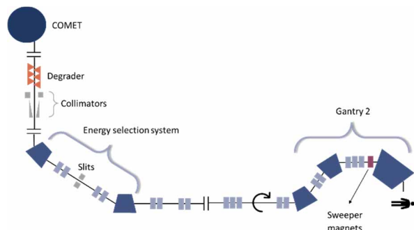
Figure 1: Schematic of the PSI beamline from the cyclotron (COMET) to Gantry 2. The light blue rectangles represent the quadrupoles, the blue trapezoid the dipoles.
