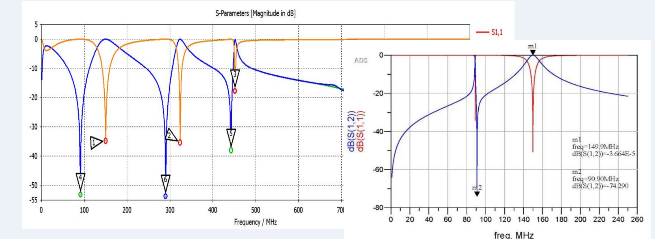
Scattering parameter of diaphragm consideration, a) Scattering parameters b) equivalent microwave circuit model
