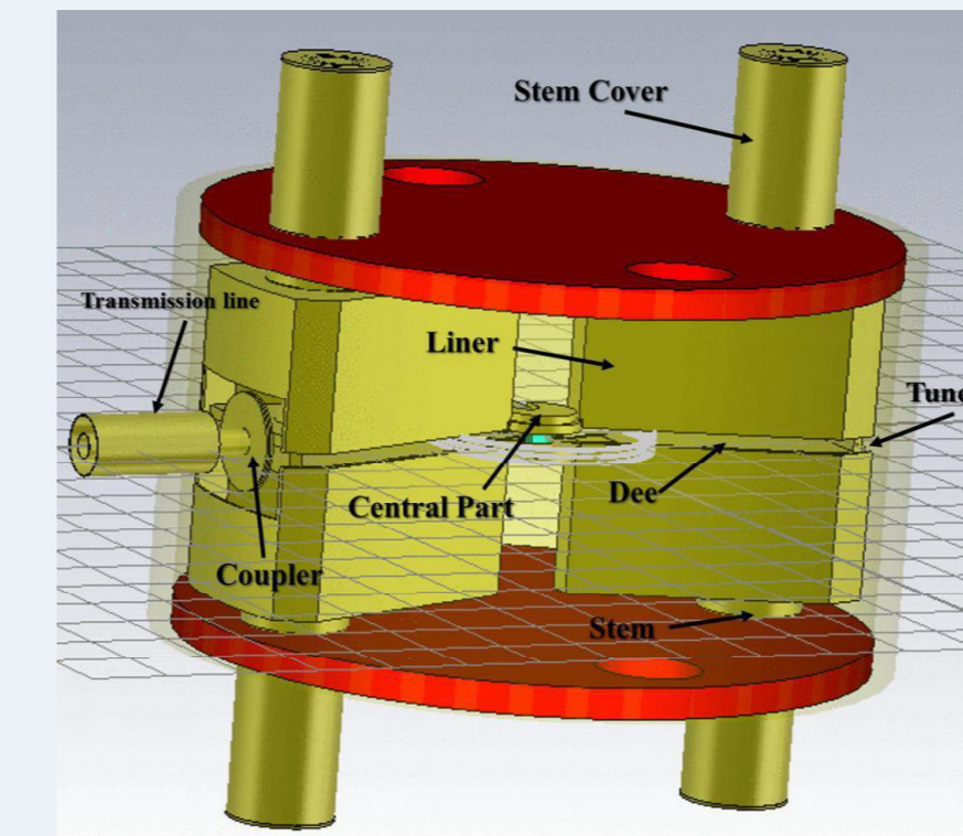
Overall structure of the RF cavity
