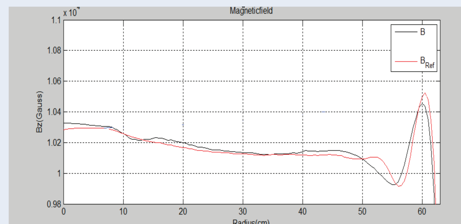
Figure 1: Average magnetic field versus radius before optimization process.
