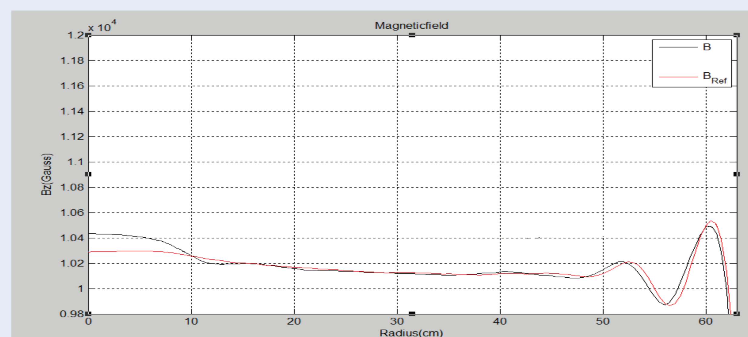
Figure 3: Average magnetic field versus radius after optimization process.
