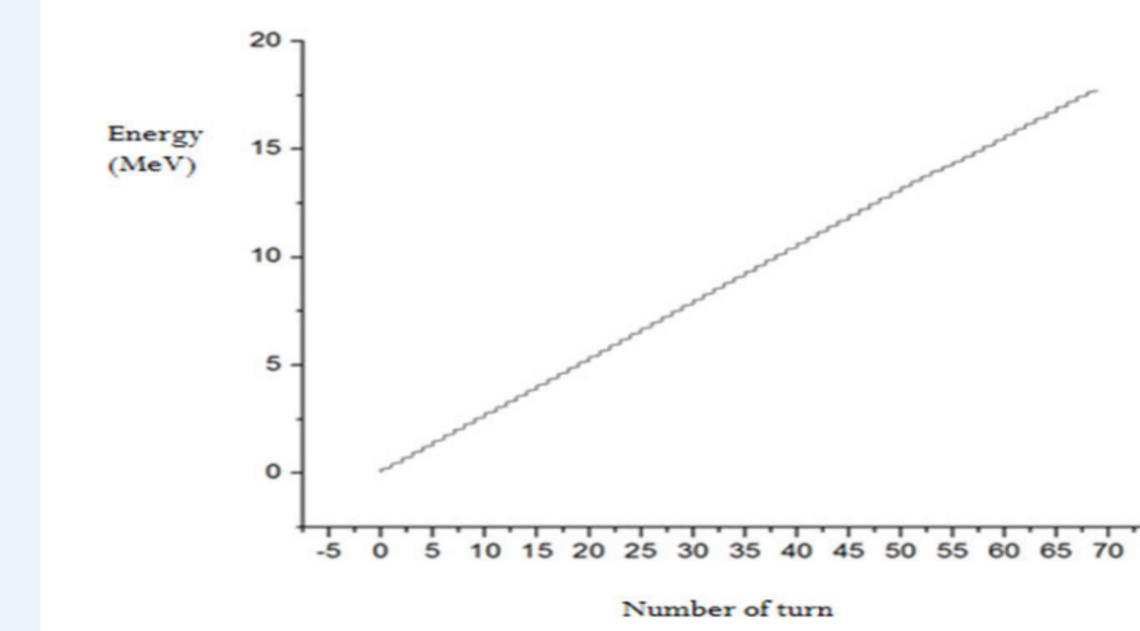
Figure 7: Kinetic energy versus number of turns.
