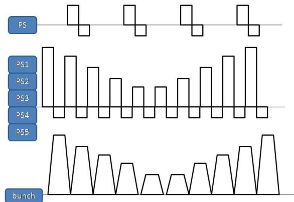
Figure 3: Sketch of ten electron bunches generated by five independent HV power supplies with the help of delay trigger.
