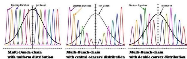
Figure 4: The longitudinal distributions of ion bunch and electron multi-bunch with different interval.
