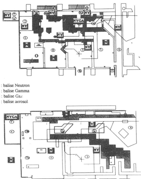
Fig.6 Layout of radiological 'balises' for SPIRAL.
