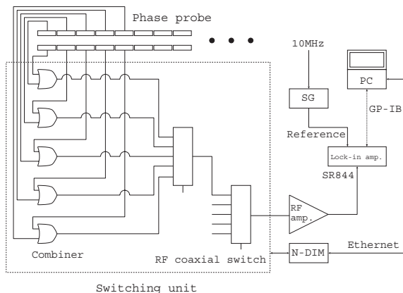
Figure 6: Schematic diagram of measuring system for phase probe.
