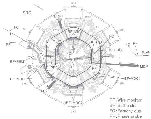
Figure 1: Entire map of beam diagnostic probes on SRC.
