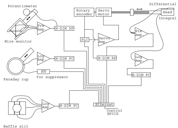
Figure 2: Schematic diagram of measuring system for wire monitor, faraday cup, baffle slit, and radial probe.
