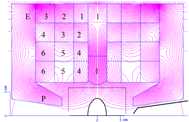
Figure 3: Schematic structure of the 18 GHz cusp ECRIS magnet and the field line contour plot.
