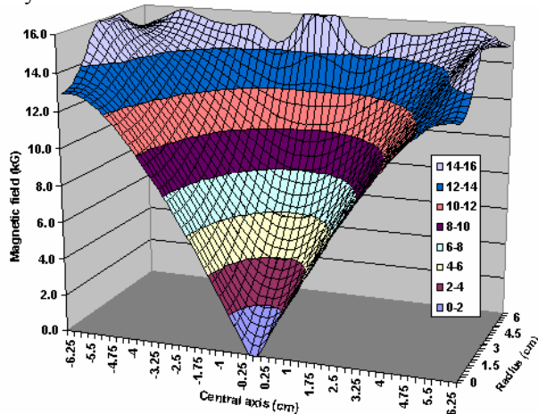
Figure 4: The 3D field plot of the 18 GHz PM cusp ECRIS.
