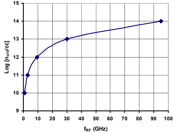
Figure 1: Critical plasma density vs. RF frequency plot.
