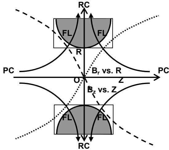
Figure 2: A scheme to produce new CMF due to PM ring. It may be a rectangle-ring instead of the shaded one.
