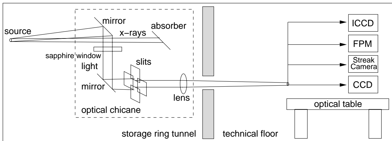
Figure 2: Schematic layout of the Optical Diagnostic Beamline viewed from side on.
