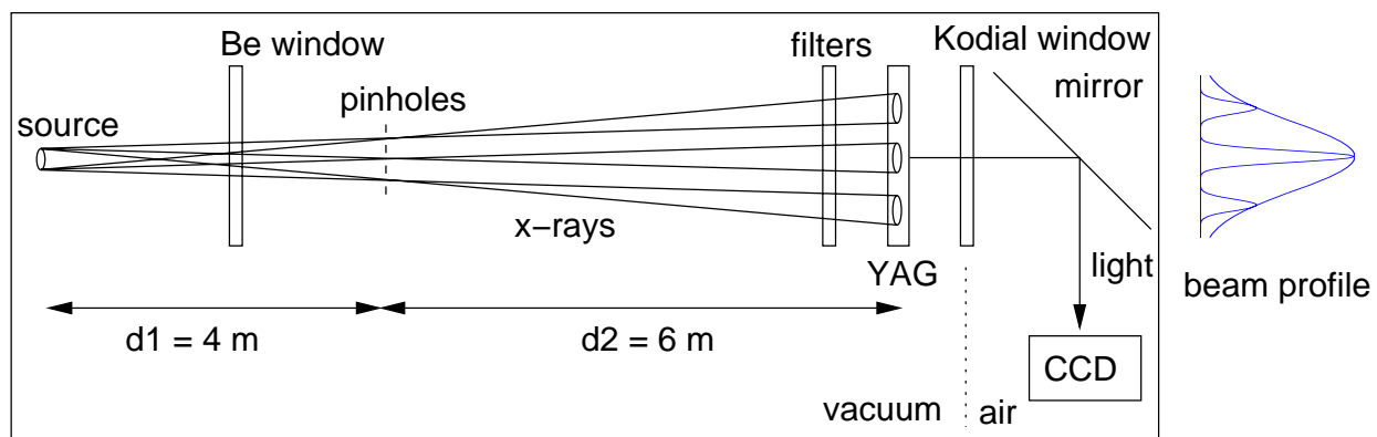
Figure 1: Schematic layout of the X-Ray Diagnostic Beamline viewed from side on.
